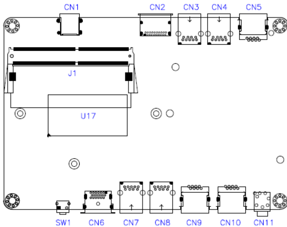
MBD642 – top and I/O
