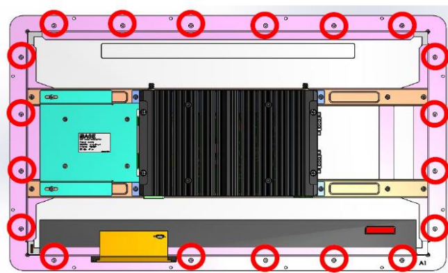
OFP-2100/2101-PC (M3 Screw *19PCS)
