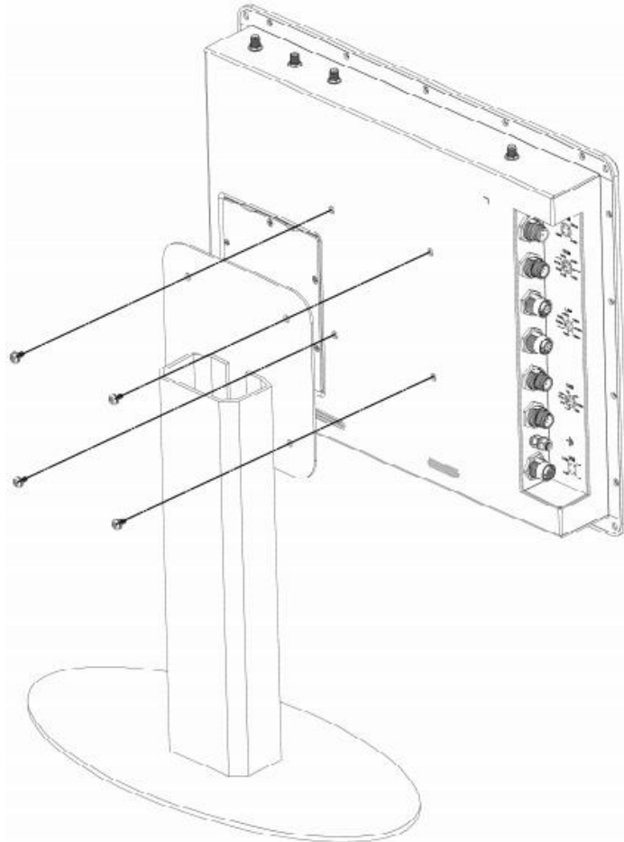
Picture of MPPC1501PC
