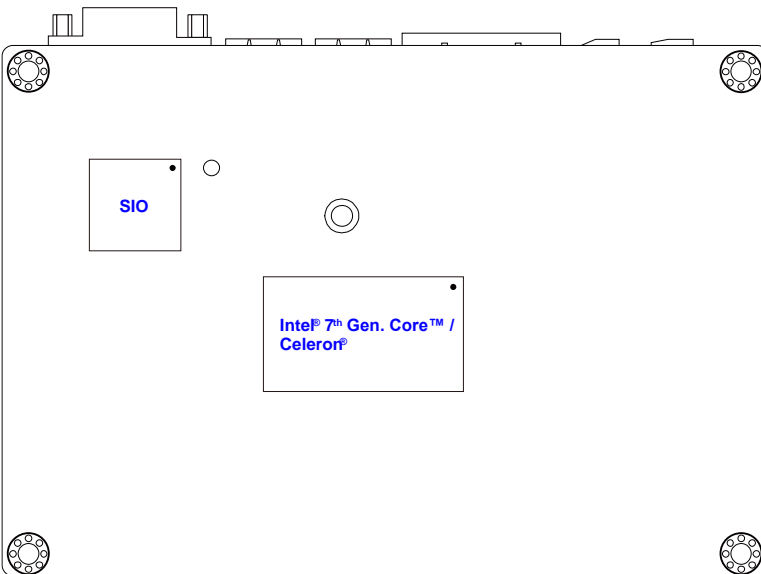
Board diagram of IB916
