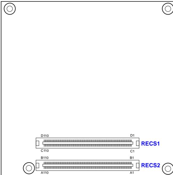
Board diagram of ET975
