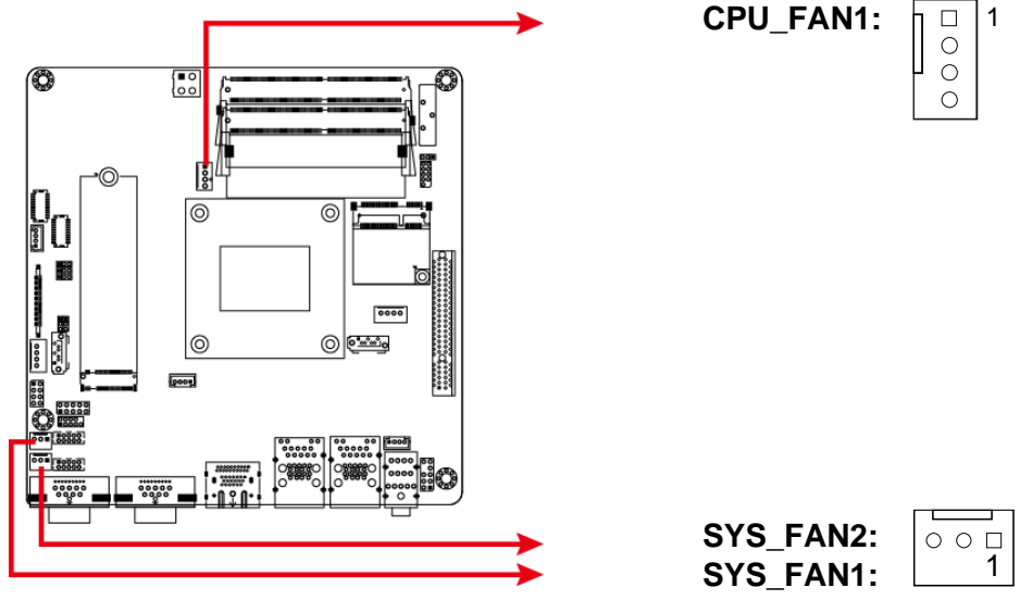
CPU_FAN1: CPU Fan Power Connector
