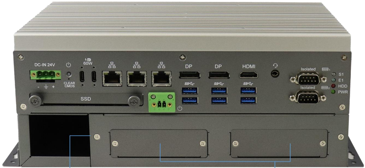
Supports different types of Fieldbus through expansion slot. Such as CAN Bus, COM and LAN...
