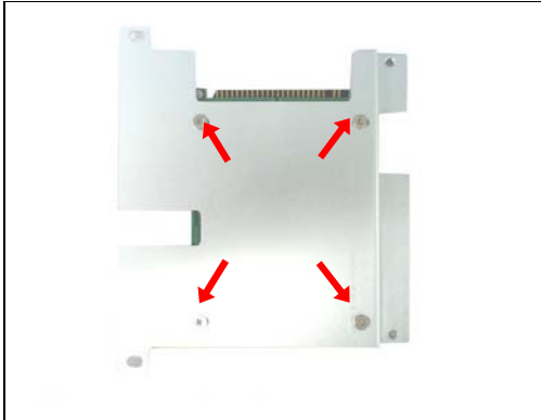
Fig. 8-1 Fasten the four screws to lock HDD and bracket together.
