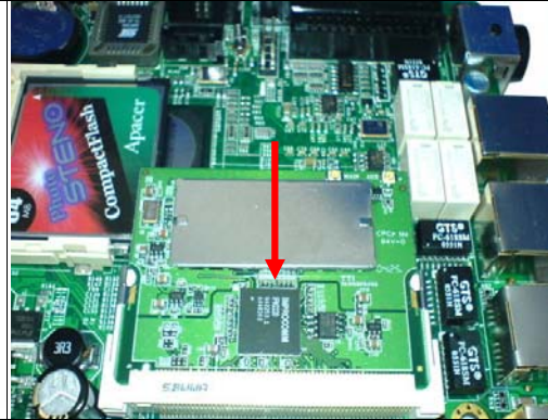
Fig. 7-2 Install the Mini-PCI card.
