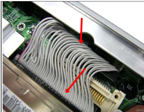
Fig. 8-3 Connect IDE cable between 3.5" HDD and IB798.
